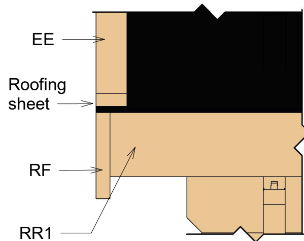
3) Roof Reinforcement
